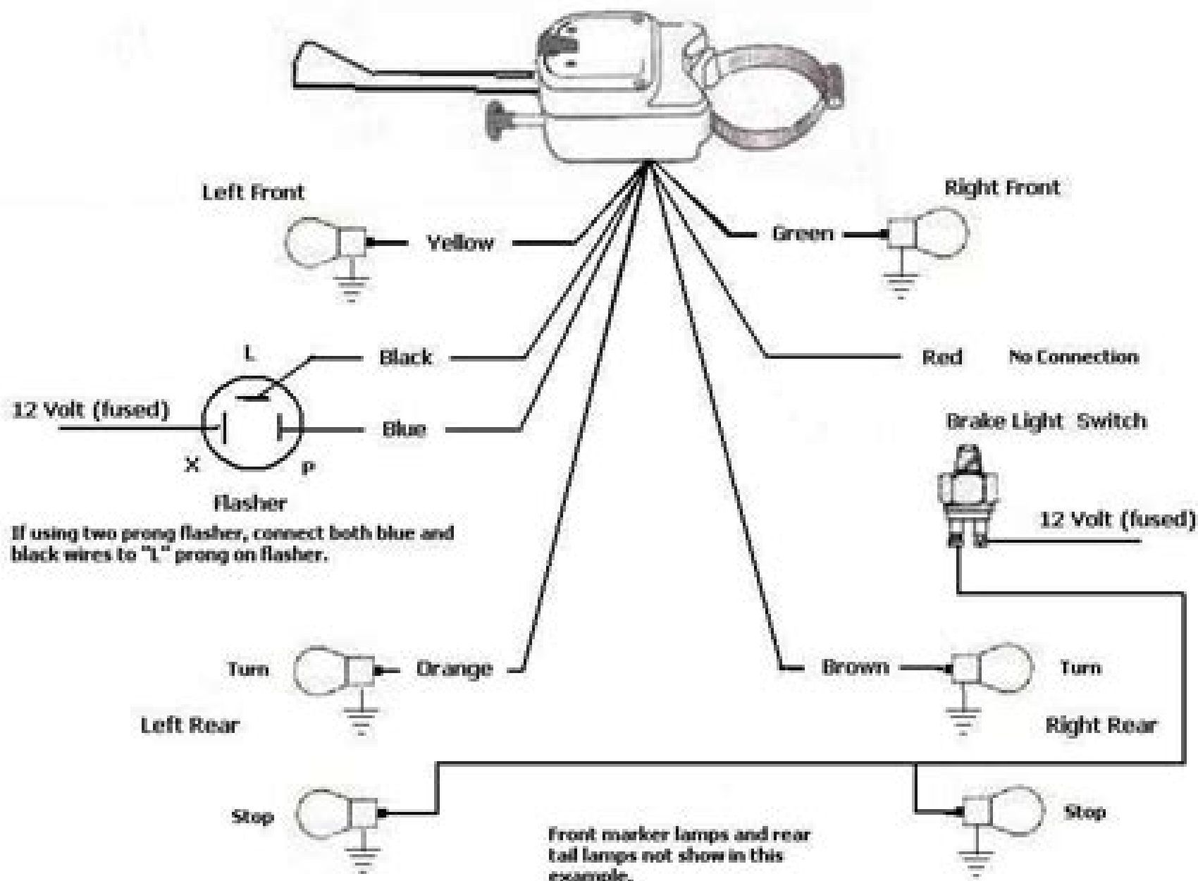
After Market (Chinese) Turn Signal Switch Wiring With sepearte stop lamps
