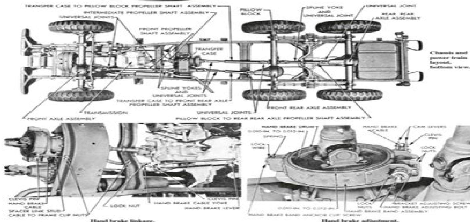
Dodge WC-43 1 1/2-ton 6x6 truck, chassis.
