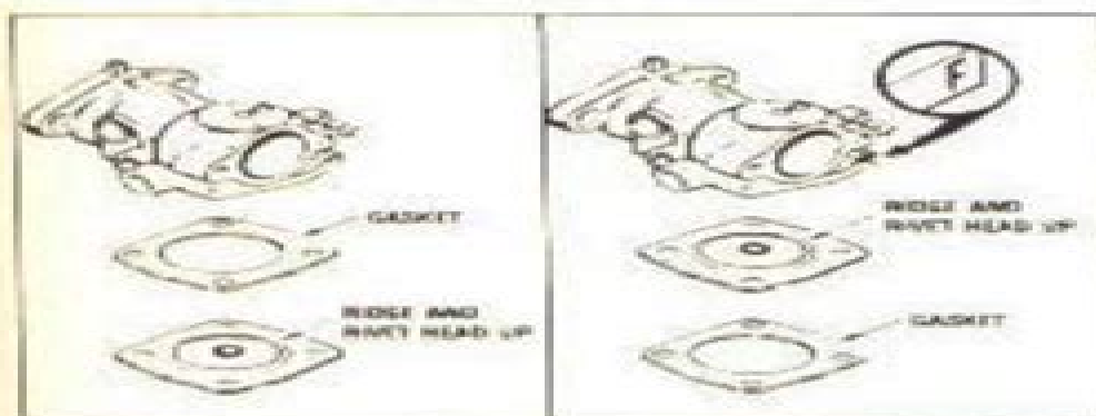
Fig. T2A—Illustration showing correct position of diaphragm on carburetors unmarked and marked with a "F".
