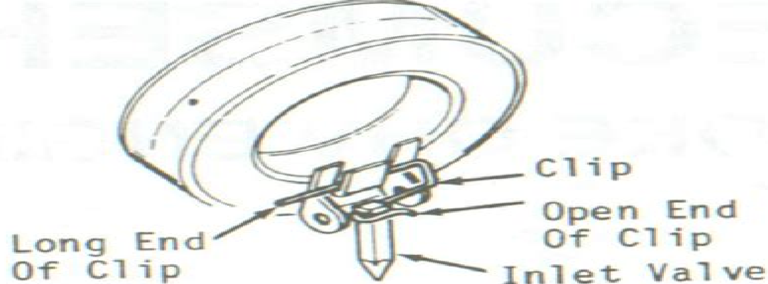
Fig. T303—Install inlet valve clip so long end points toward intake end of carburetor.
