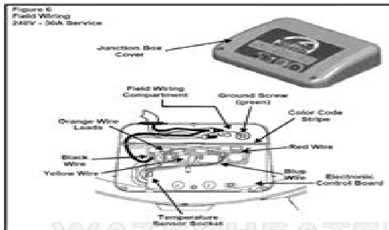
Wiring Diagram 240 Volts Only
