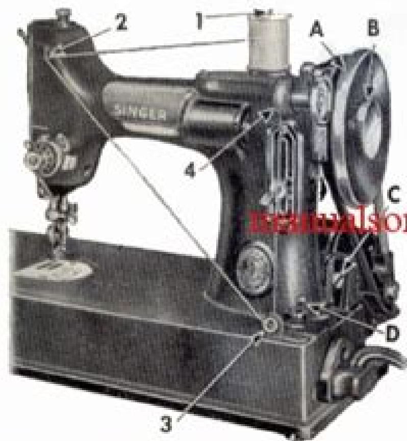
Fig. 9. Winding the Bobbin
