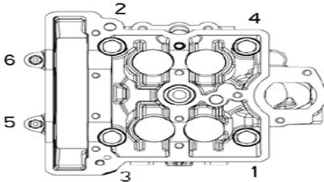
CYLINDER HEAD TORQUE SEQUENCE
