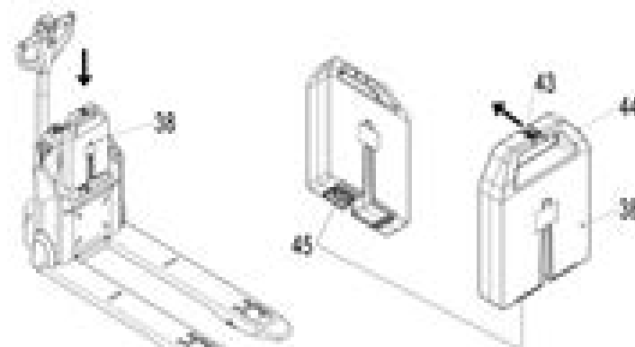
Fig. 35. Battery installation
