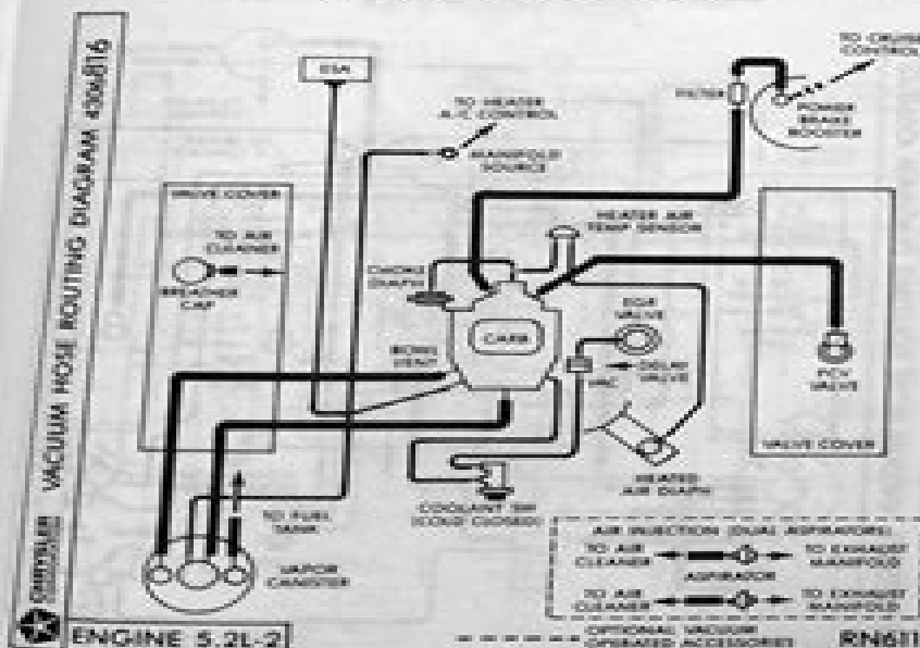
Fig. 13—Vacuum Hose Routing Label 5.2L-2 Canadian ESA with Catalyst and Aspirator
