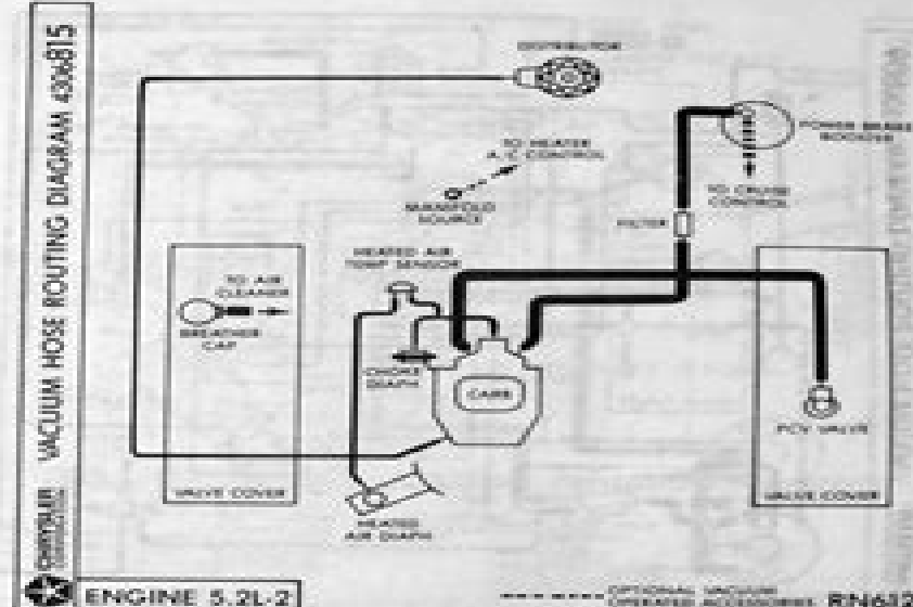
Fig. 14—Vacuum Hose Routing Label 5.2L-2 Canadian without Catalyst and without ESA
