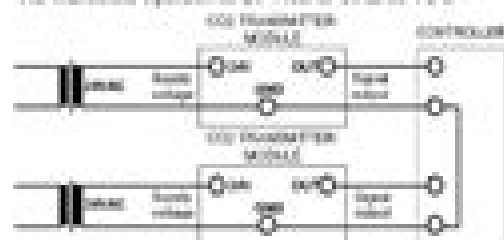
Figure 2 Connection of Separate AC Supply (Recommended)
