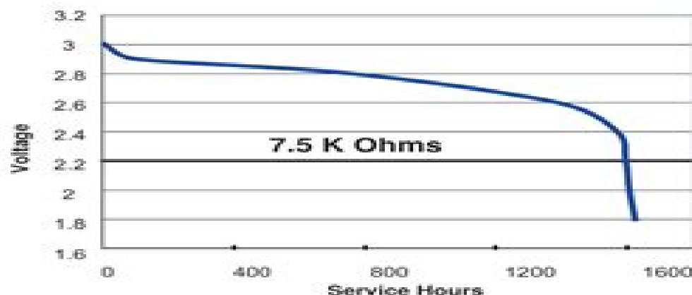
Typical Discharge Characteristics at 21°C (70°F)
