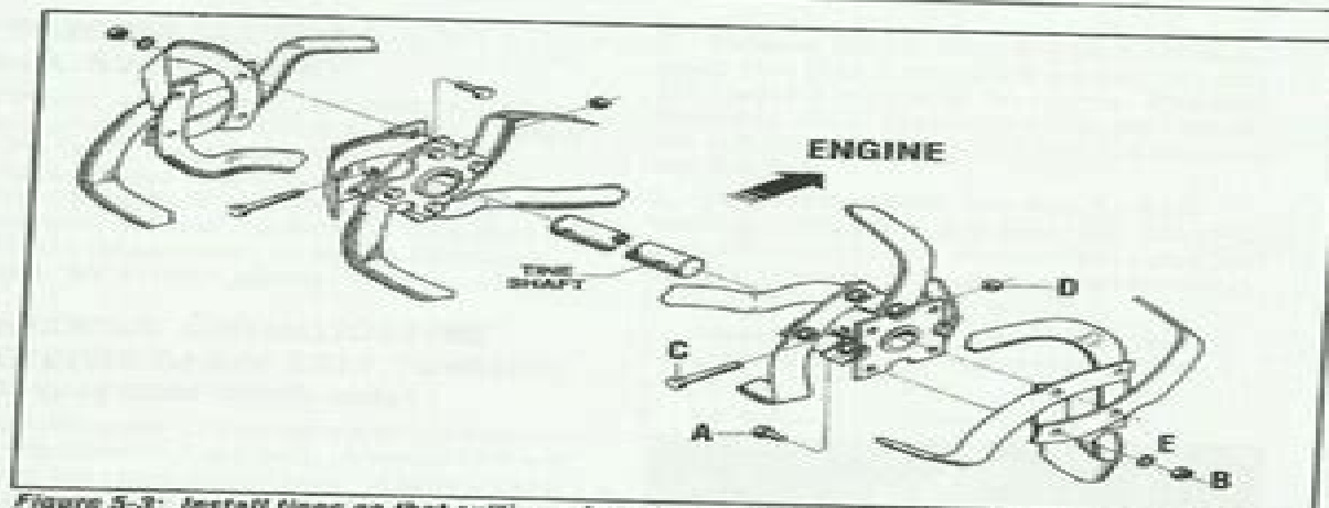
Figure 5-3: Install lines so that cutting edge of lines enter soil first when tiller moves forward.
