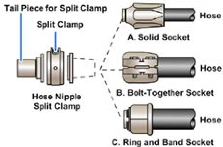
End Fitting Split Clamp to A, B, or C
