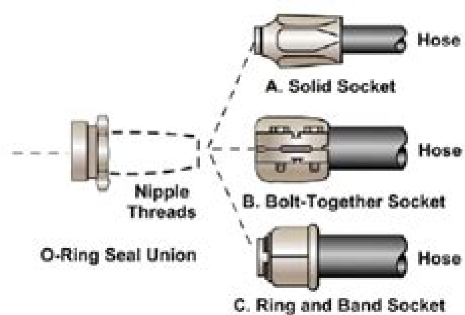
End Fitting O-Ring Seal Union to A, B, or C
