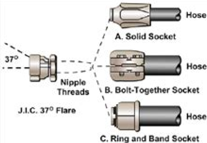
End Fitting 37° J.I.C. to A, B, or C
