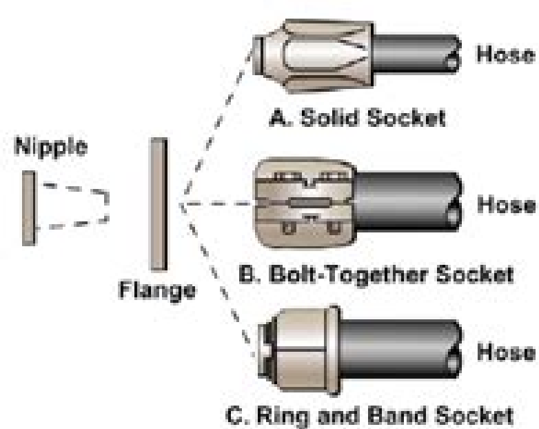
End Fitting Flange to A, B, or C
