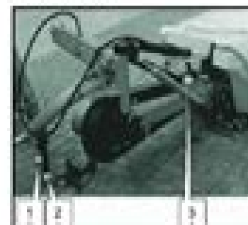
Fig. 62 Parked machine (stand lowered)
