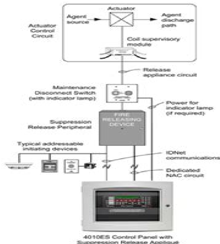
4010ES Release Control Simplified Block Diagram
