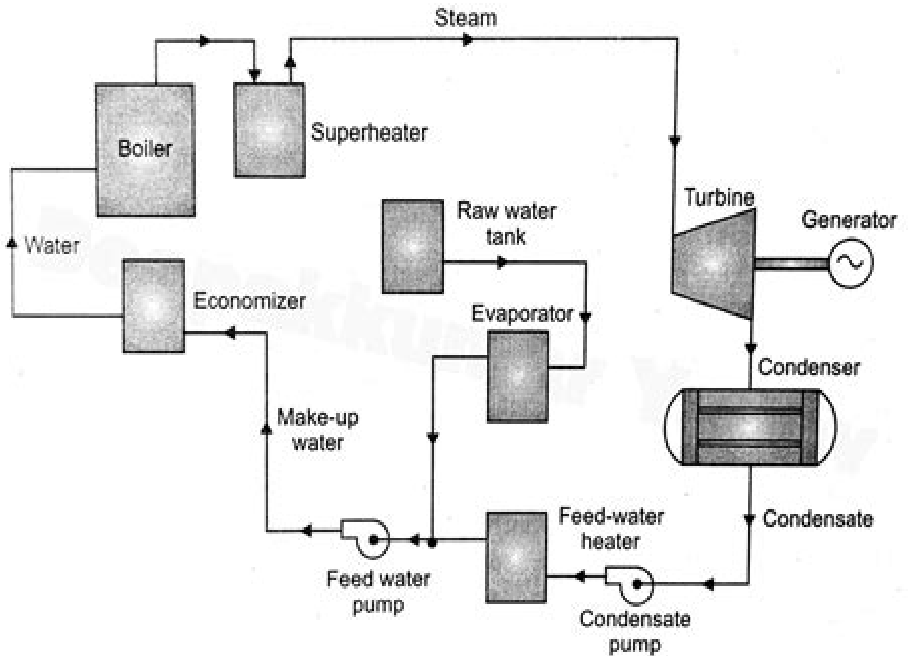
Feed Water and steam flow circuit for a Boiler turbine unit
