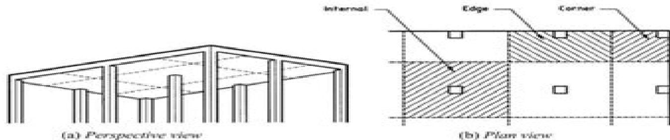
Figure 3.1 Concrete Slab on Columns
