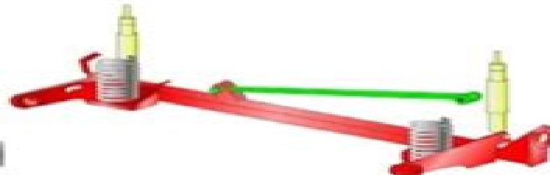
Left: Solid axle rear suspension with leaf springs. Right: Solid axle "trailing arm" rear suspension for a front-wheel-drive model. Note the track bar directly above the axle.
