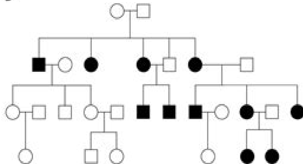
Mitochondrial
