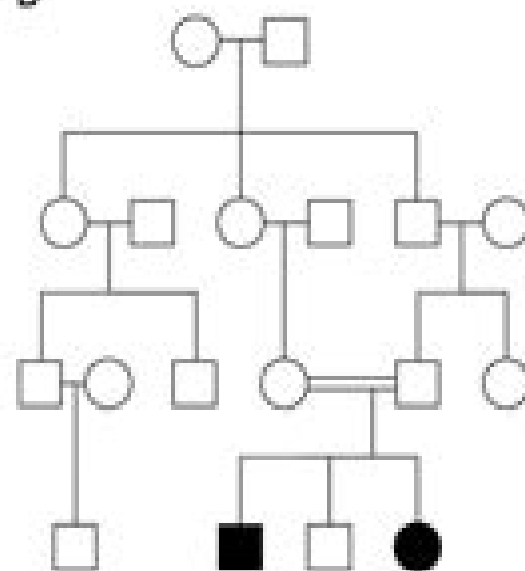
Autosomal recessive
