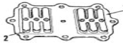
Fig. S24-5—View showing reed plate (1) and reed valve (2) assembly used on DT6 and DT8 models.
