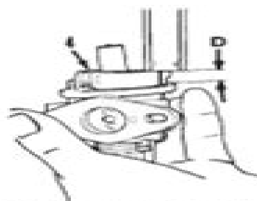
Fig. S24-2—For proper float level, adjust distance (D) from top of carburetor body flange to base of float (4). Refer to text for specifications.
