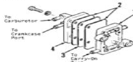
Fig. S24-3—Exploded view of diaphragm type fuel pump.
