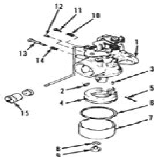
Fig. S24-1—Exploded view of Mikuni BY-18-13 carburetor used on DT5 models. Carburetors used on DT6 and DT8 models are similar.
