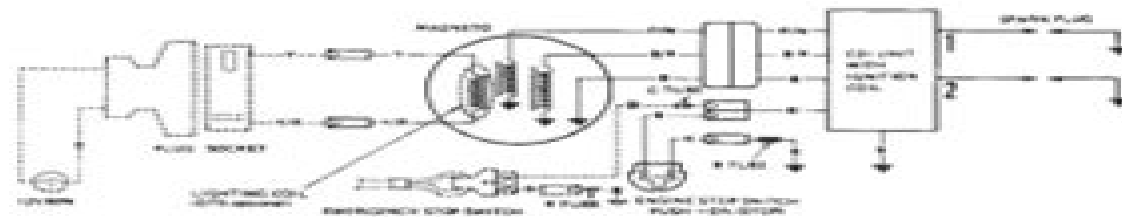
Fig. S24-6—Wiring diagram typical of all models.
