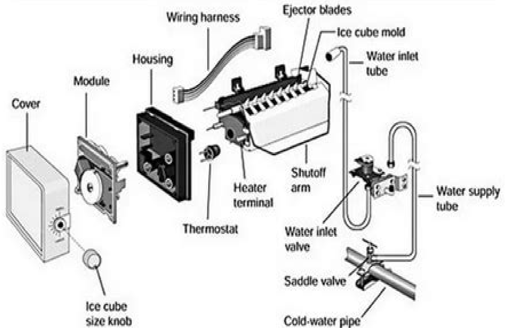
Ice Maker Parts Identification Illustration
