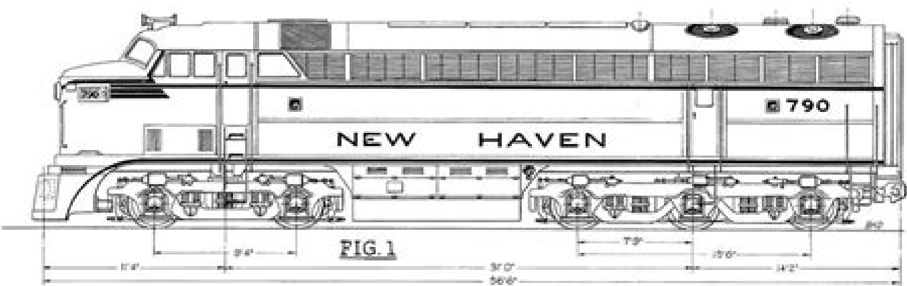
FAIRBANKS MORSE "C-LINE" DIESEL
