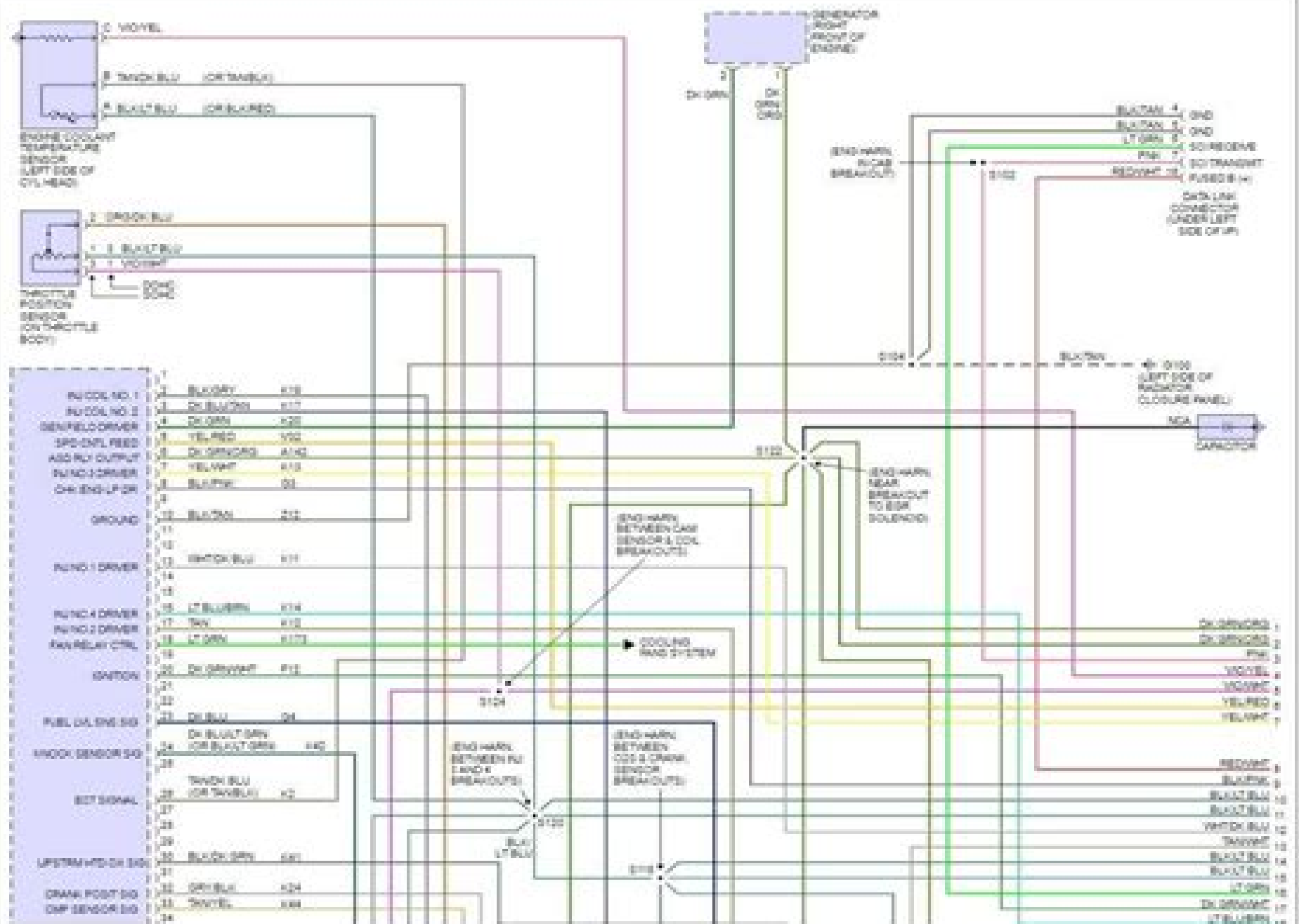
Fig 1: 2.0L Engine Performance Circuits (1 of 3)
