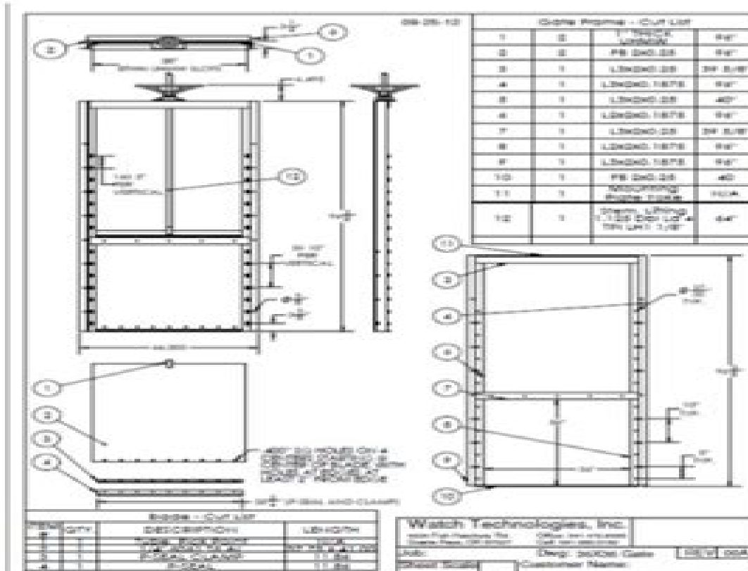
Figure 1. Typical Flush Mount Manually Actuated Gate
