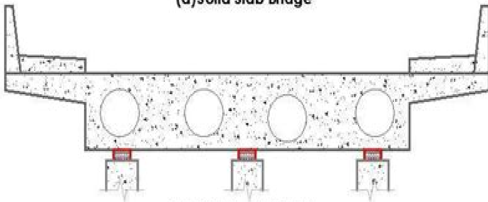
(b) Voided Slab Bridge
