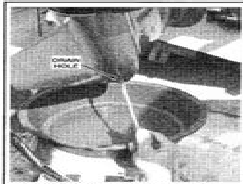
Fig. 22 When draining the lower unit, ensure it is fully tilted and a drain pan of adequate capacity is placed to catch the lubricant
