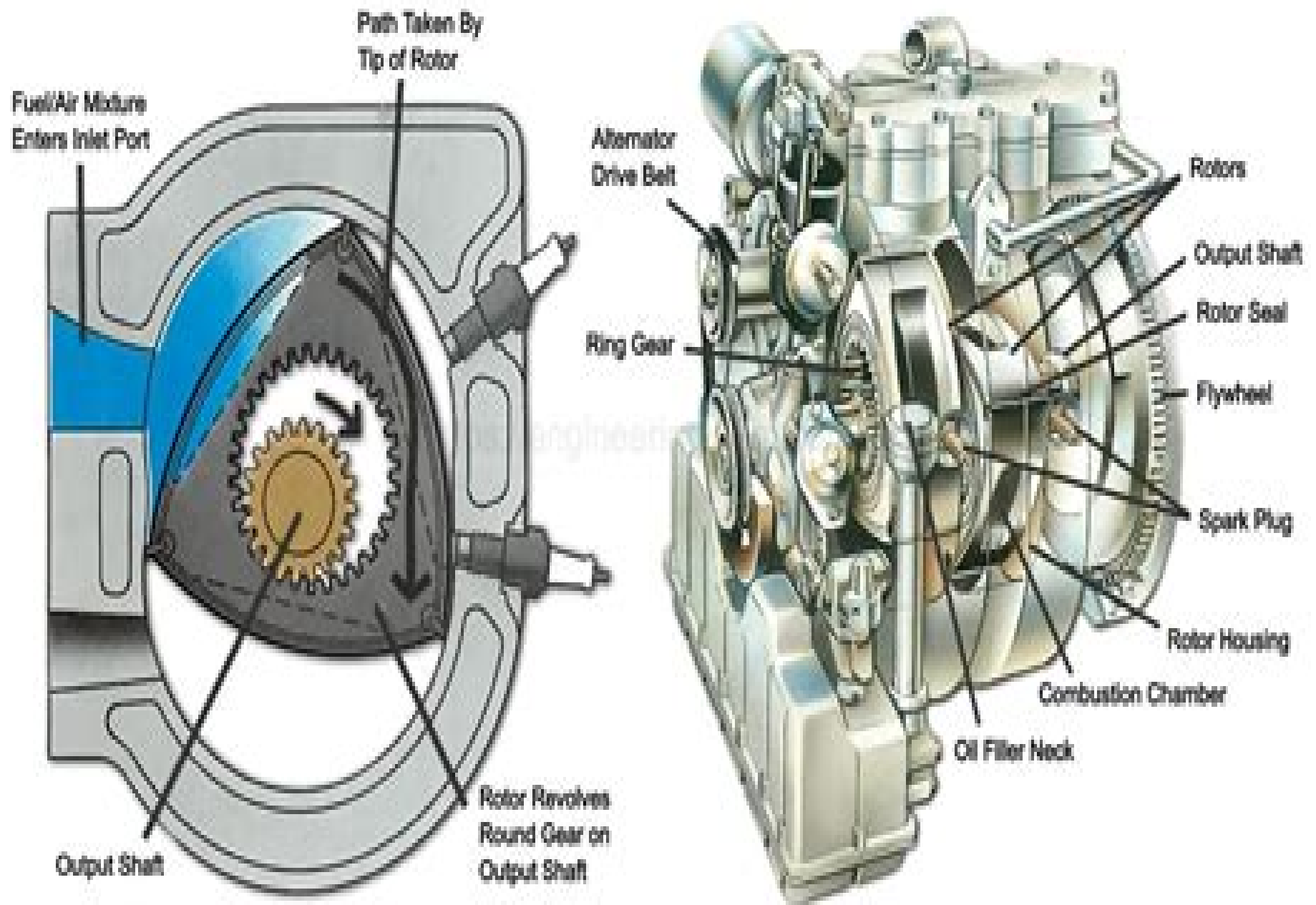
Wankel Engine (Rotary Wankel Engine)
