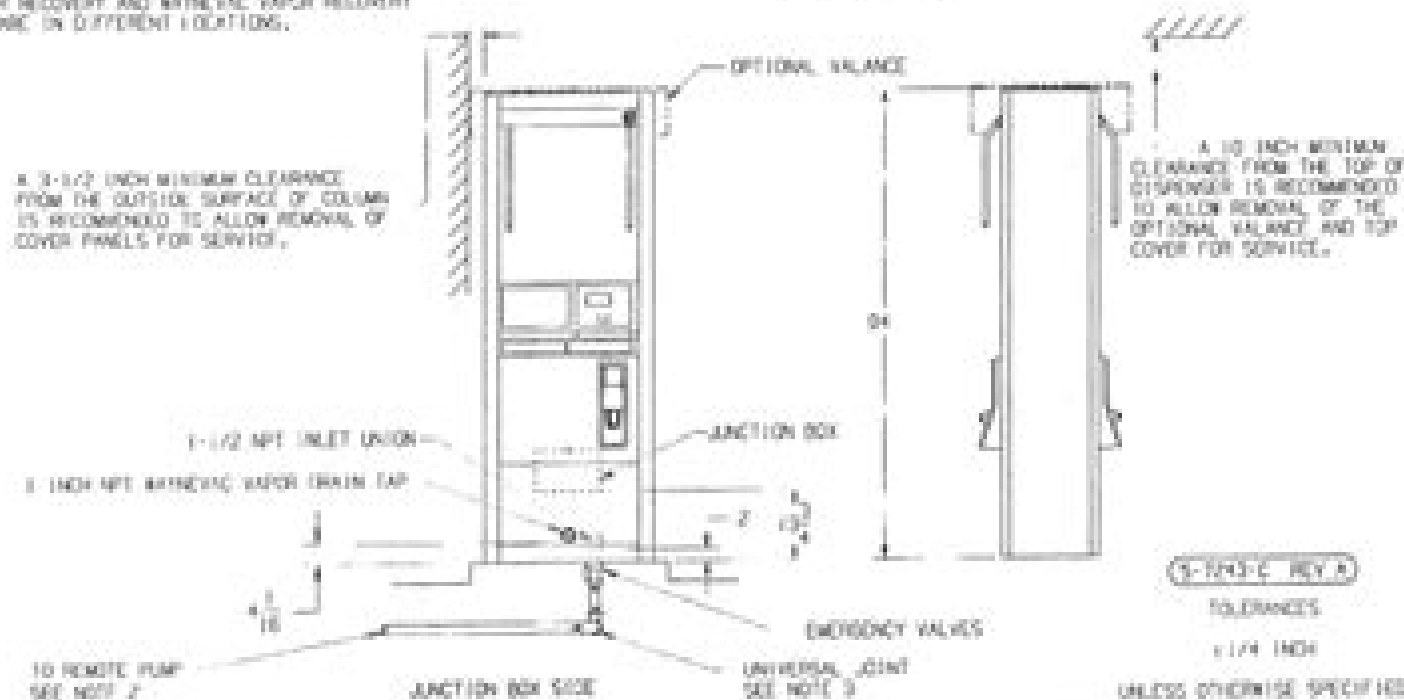
BASE DIMENSIONS
