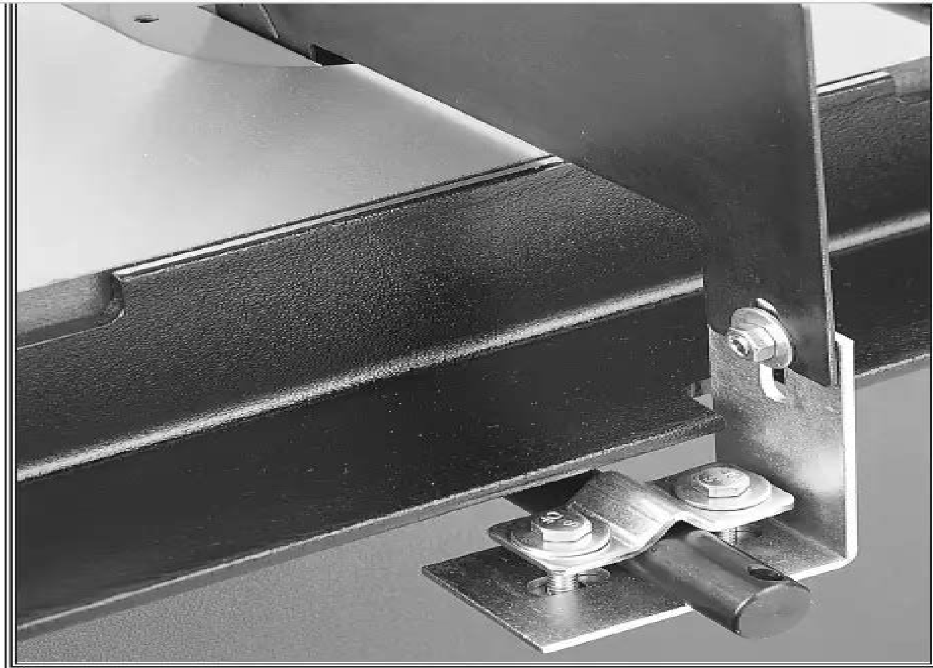
Figure 8. Rail and guard bracket installation.
