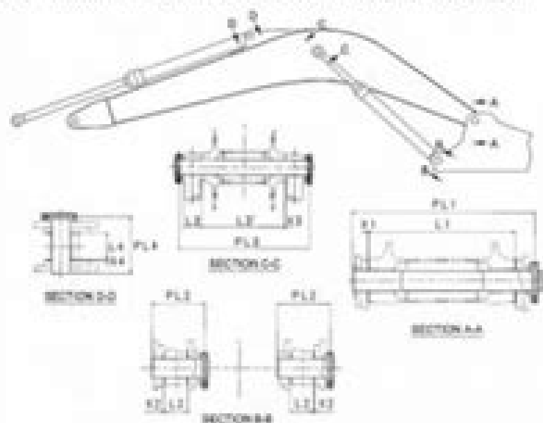
Fig. 2.22 Clearance in thrust direction on the boom cylinder installation section
