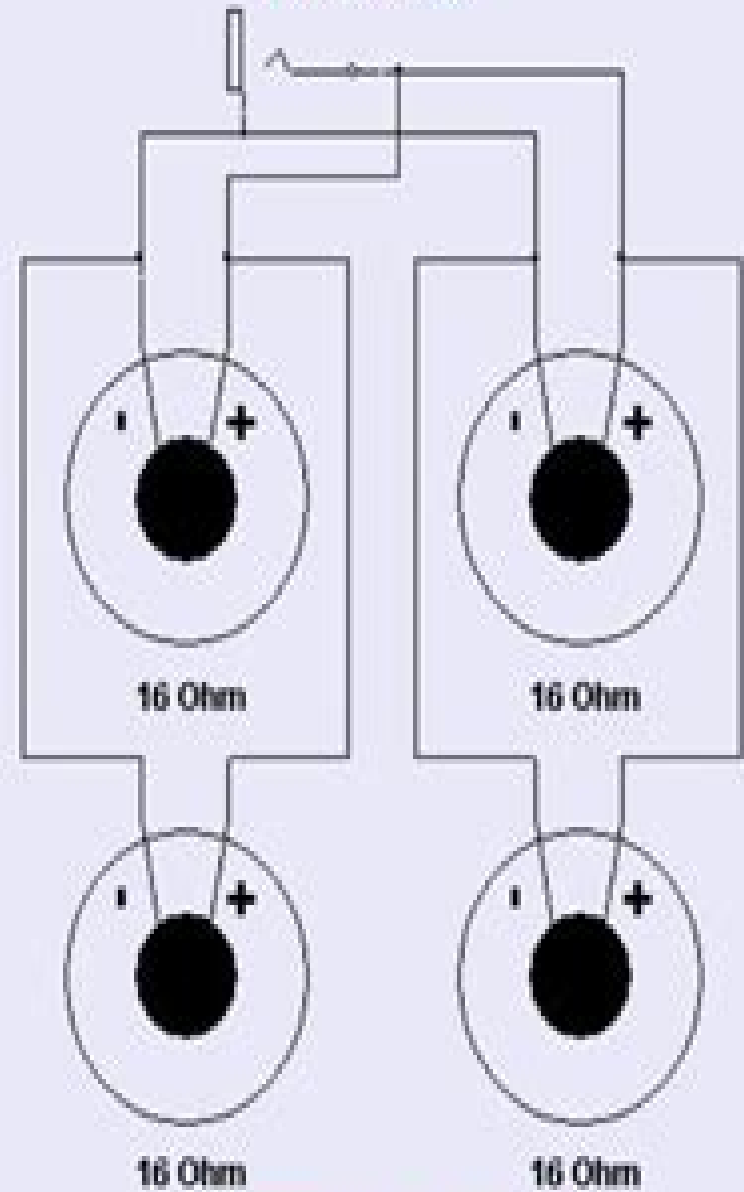
PARALLEL WIRING
