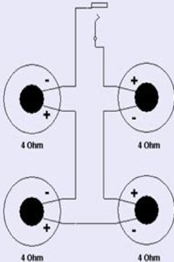
SERIES WIRING
