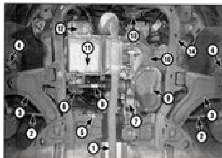
Front underbody view of a 1.2 litre model
