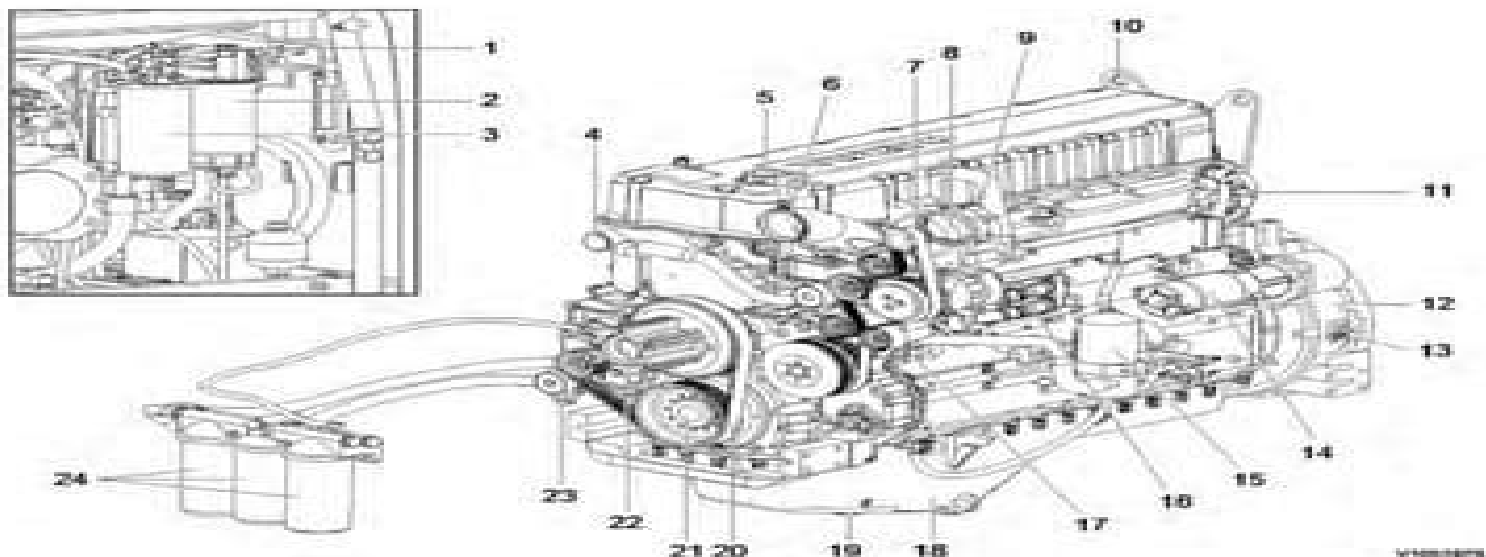
Figure 1 Engine, structure
