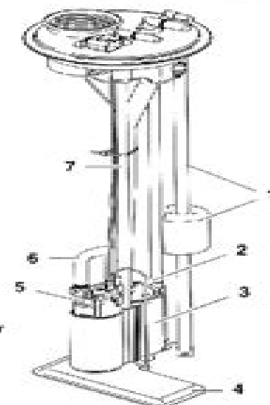
Figure 4-5. Fuel Pump/Filters/Fuel Level Sender Assembly
