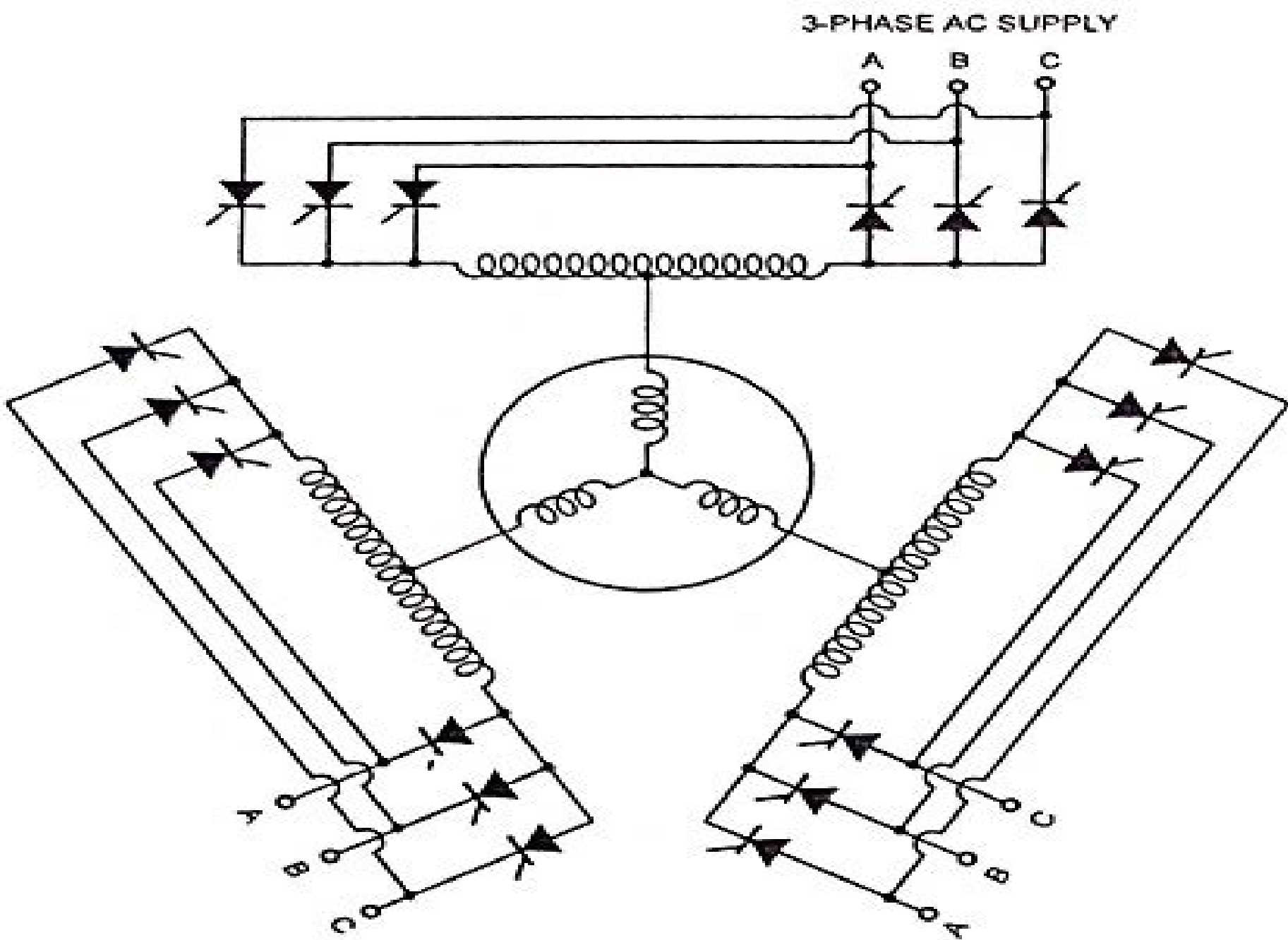
Fig. 27.36 3-Phase Cycloconverter
