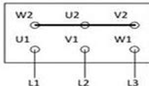
Terminal Connections
