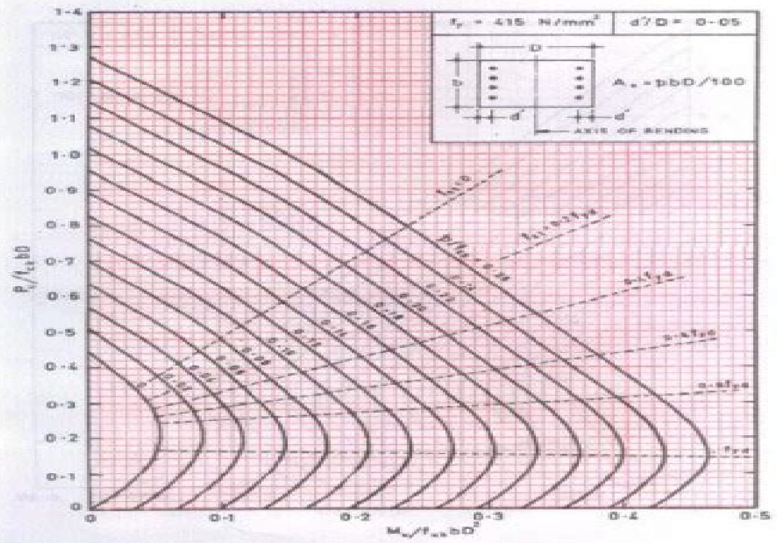
Chart 31 COMPRESSION WITH BENDING — Rectangular Section — Reinforcement Distributed Equally on Two Sides
