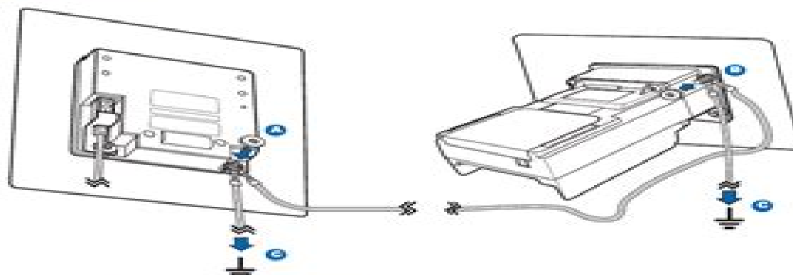
Figure 11 Grounding the UX300 and PIN Pad Units
