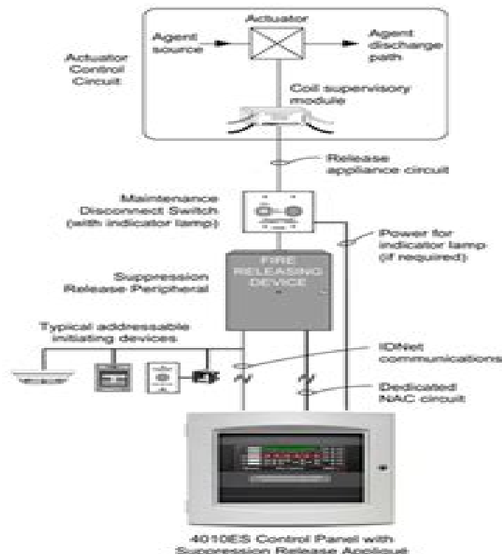
4010ES Release Control Simplified Block Diagram
