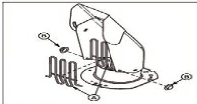
Figure 1. Remove Chute Guard A. Chute Guard B. Push Nuts
