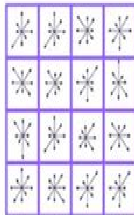
Keypoint descriptor
