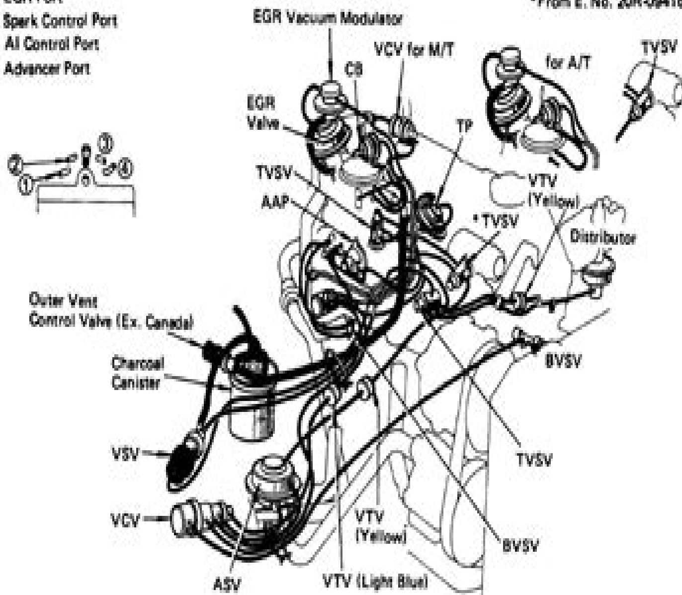
Fig. 59: 1978 Celica & Corolla (20R Engine) Exhaust Emission System (Federal)
