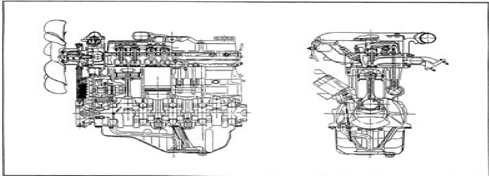
1DZ-4I Engine
