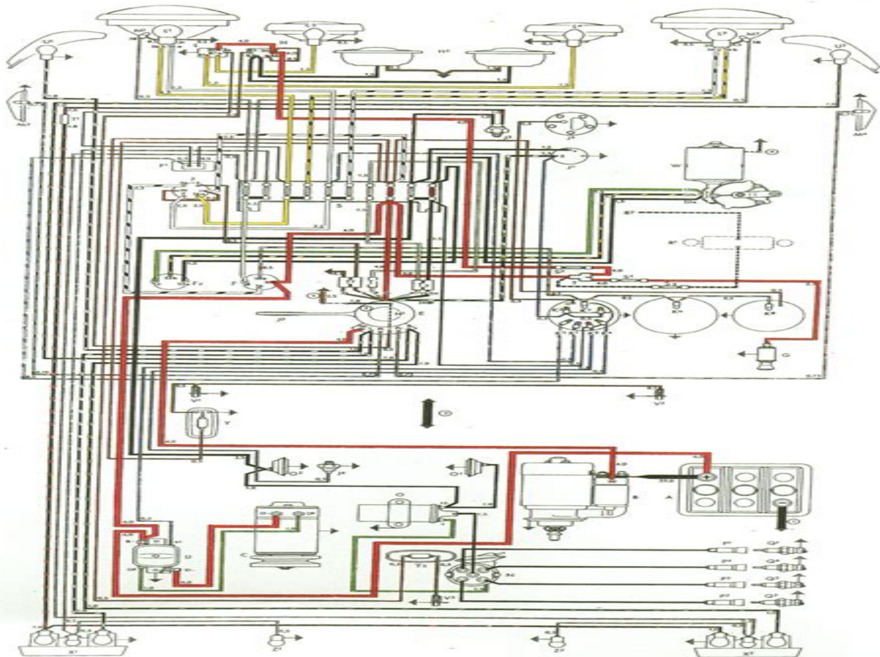
Wiring Diagram VW 1500 — Karmann Ghia Models (from May 1964, Chassis No. 0 425 853)
