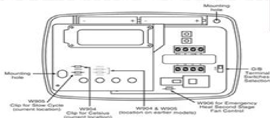
Figure 1. Thermostat base
