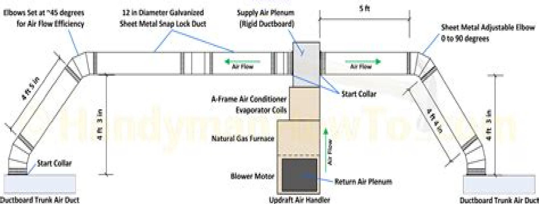
Attic Air Handler Ductwork Side View
