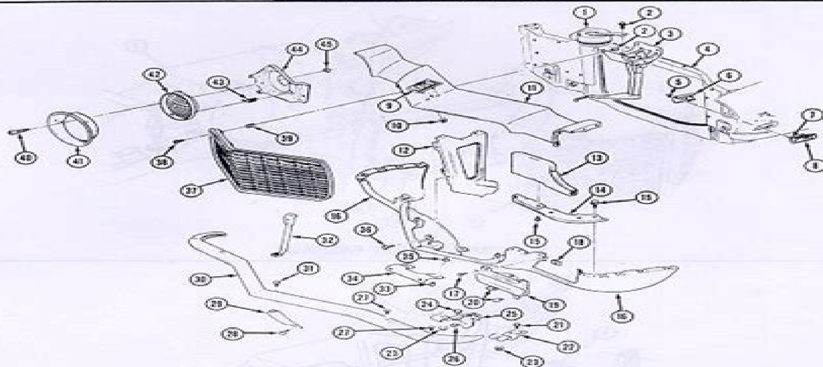
1971-72 GRILLE AND BUMPER (EXC. R.S.)
