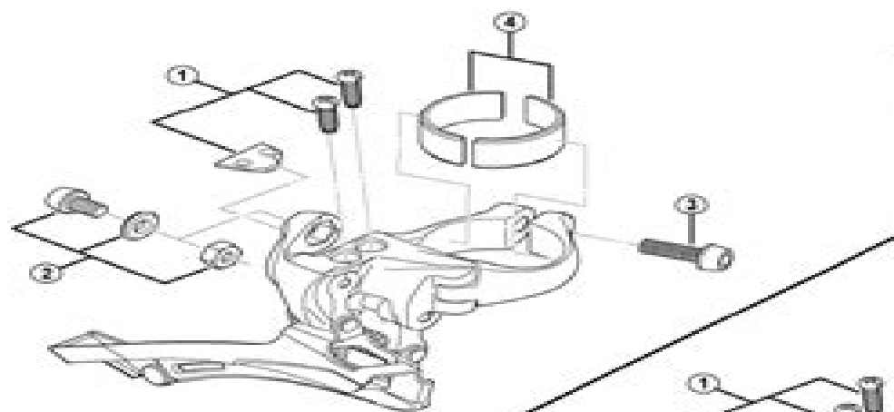
Band Type
