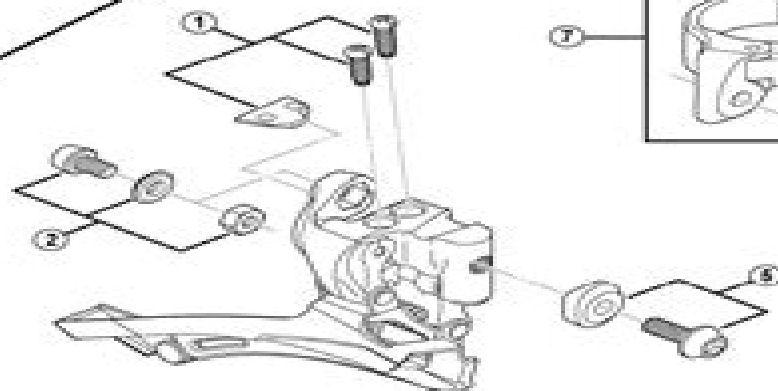
Brazed-on Type
