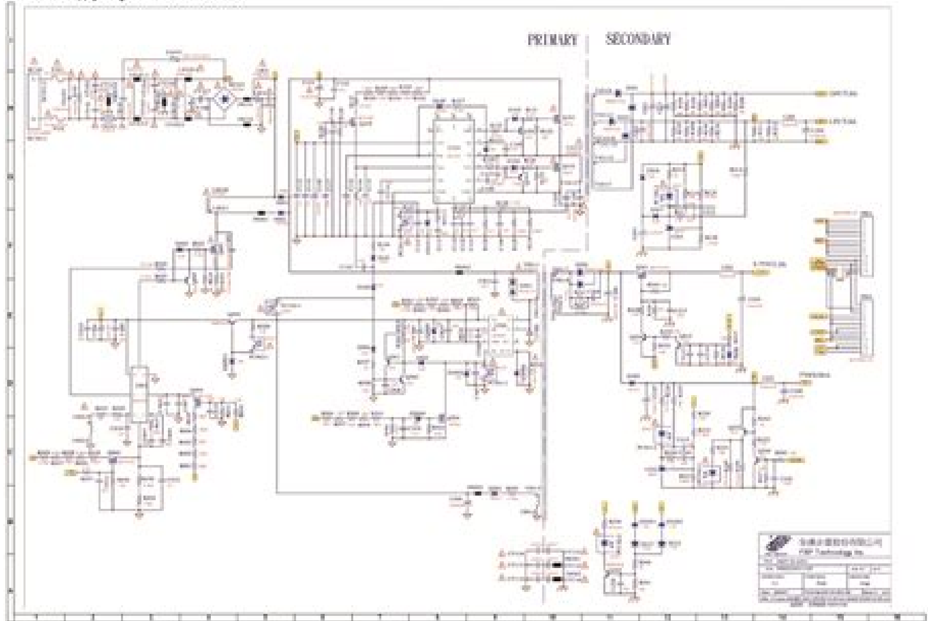
Power Supply Diagram: ACDC-CA-100W-02
