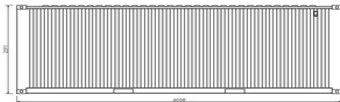
20ft Shipping Container - Side Elevation
