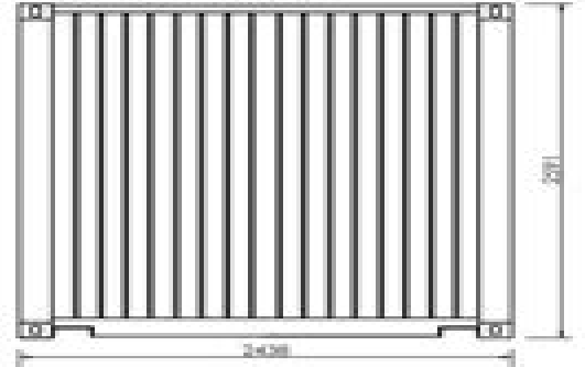
20ft Shipping Container - Door Elevation
