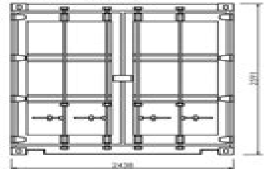
20ft Shipping Container - Door Elevation
