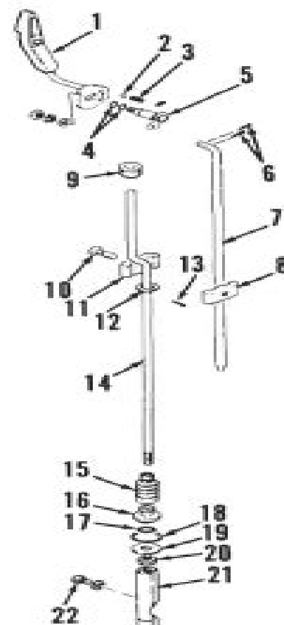
Fig. S24-19—Exploded view of shift control linkage.
