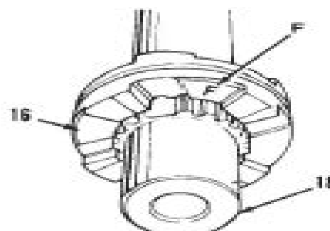
Fig. S24-18—Install dog clutch (16) on propeller shaft (18) so "F" mark (F) is toward forward gear.
